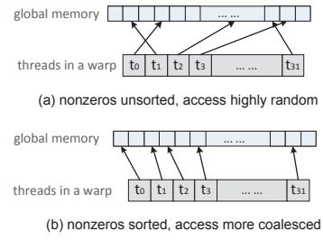
Figure 4: More coalesced memory accesses after sorting
