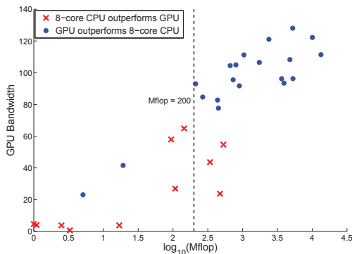
Figure 6: Relation between Mflops and GPU speedups
