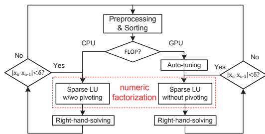
Figure 9: The proposed workflow of CPU/GPU hybrid sparse solver for circuit simulation.
